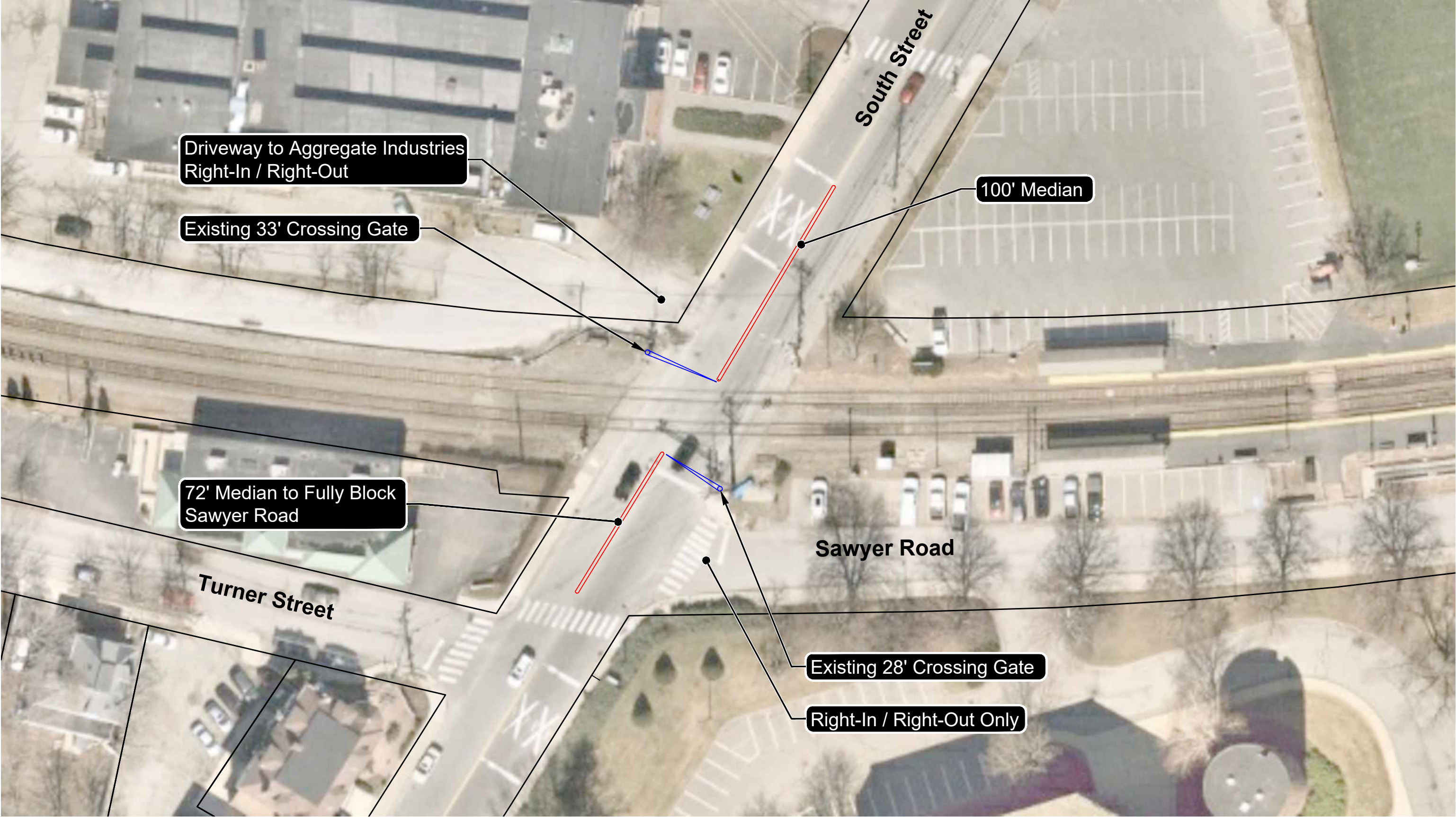
City of Waltham, Massachusetts South Street Grade Crossing Schematic Plan
